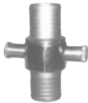
Order No: FAR-6 Female Screw x Female Instantaneous
