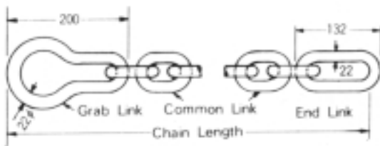
Deck Lashing Chain
